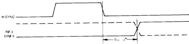
FIGURE 3 SCAN AND DATA ROW COUNTER TIMING
