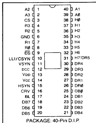
PACKAGE: 40-Pin D.I.P.
