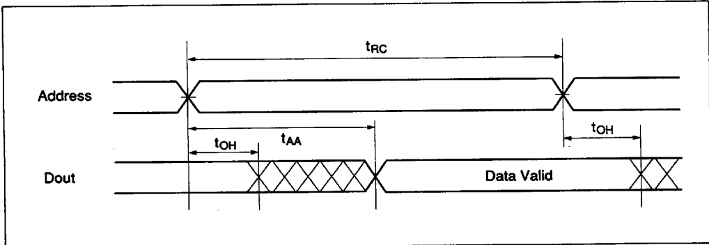
Read Timing Waveform (2) *3 *4 *6
