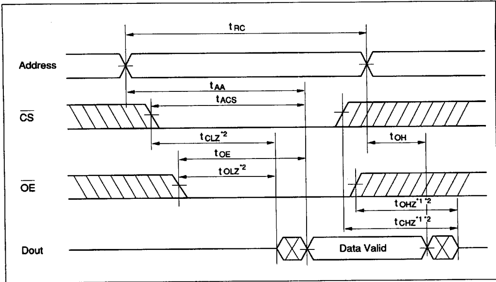
Read Timing Waveform (2) *3 *4 *6
