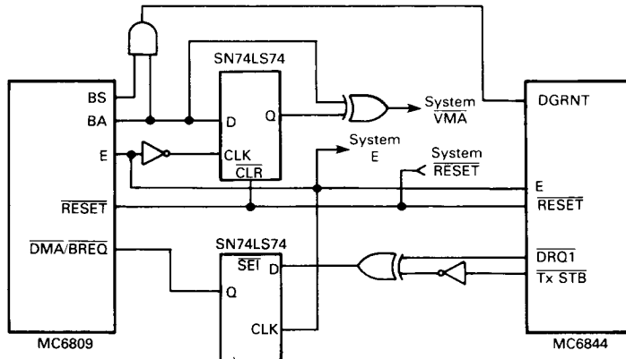
FIGURE 13 — MC6844/MC6809 INTERFACE FOR MODE 1 DMA
