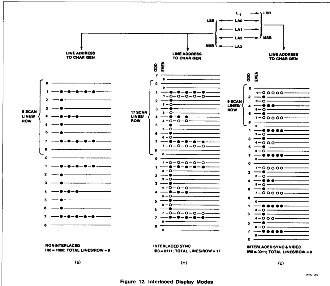
Figure 12. Interlaced Display Modes
