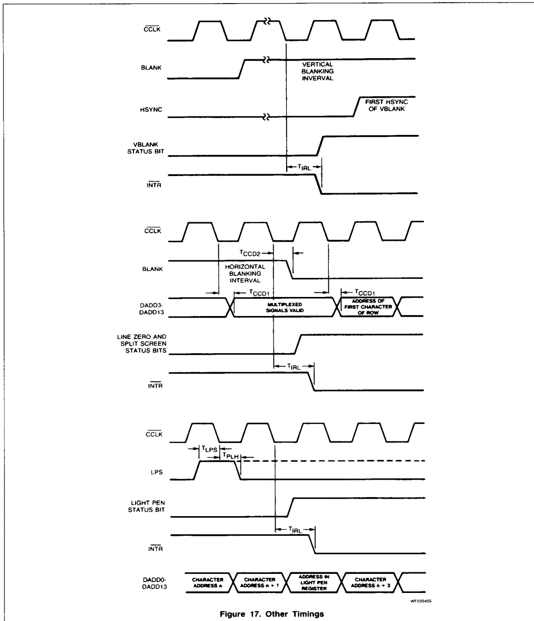
Figure 17. Other Timings
