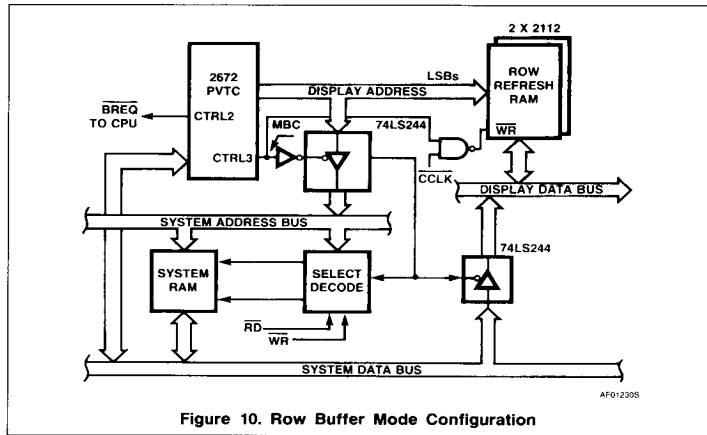
Figure 10. Row Buffer Mode Configuration
