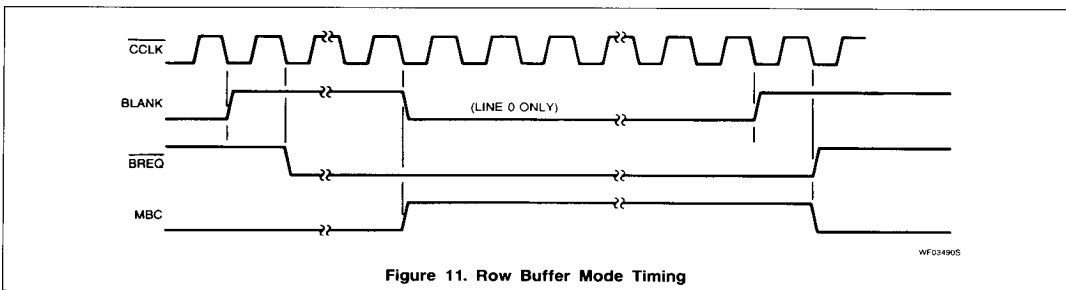
Figure 11. Row Buffer Mode Timing
