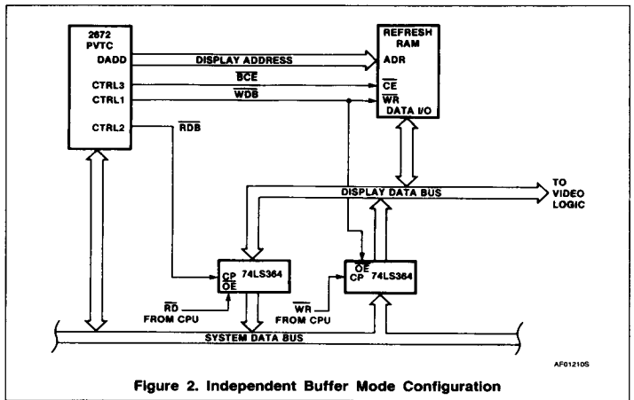
Figure 2. Independent Buffer Mode Configuration
