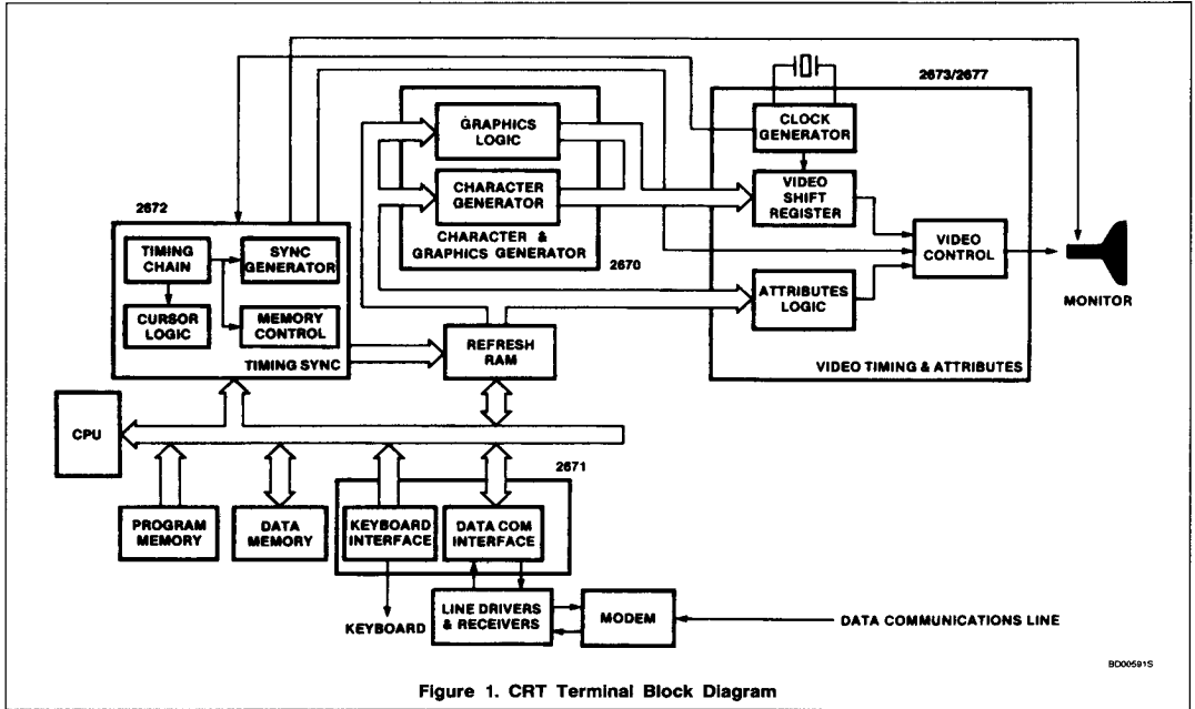
Figure 1. CRT Terminal Block Diagram
