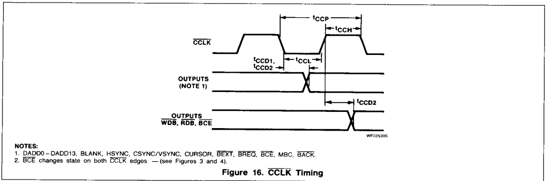
Figure 16. CCLK Timing
