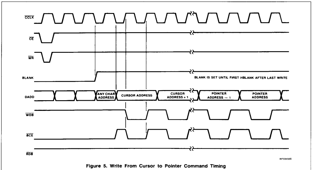
Figure 5. Write From Cursor to Pointer Command Timing
