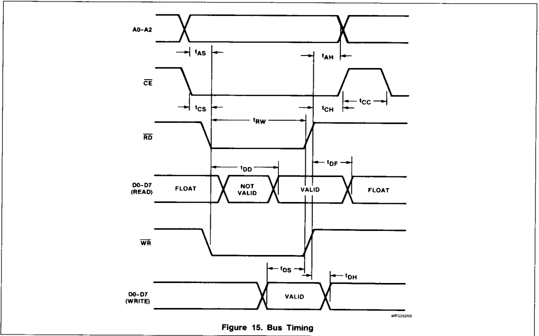
Figure 15. Bus Timing
