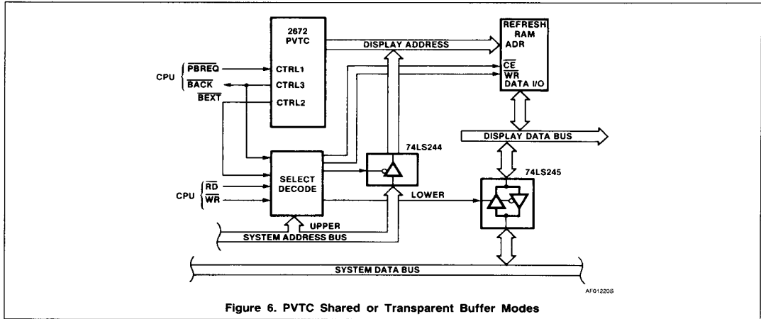
Figure 6. PVTC Shared or Transparent Buffer Modes
