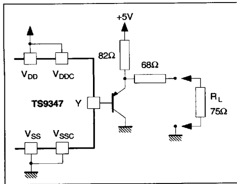
Figure 11 : Typical Application
