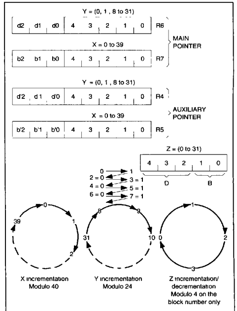
Figure 15 : Pointer Auto Incrementation
