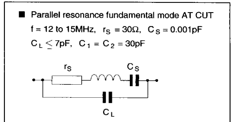
Figure 2 : Typical Crystal Parameters
