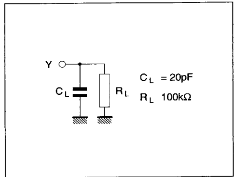
Figure 12 : Test Condition
