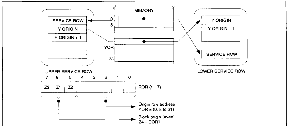
Figure 18a : Screen Format Table
