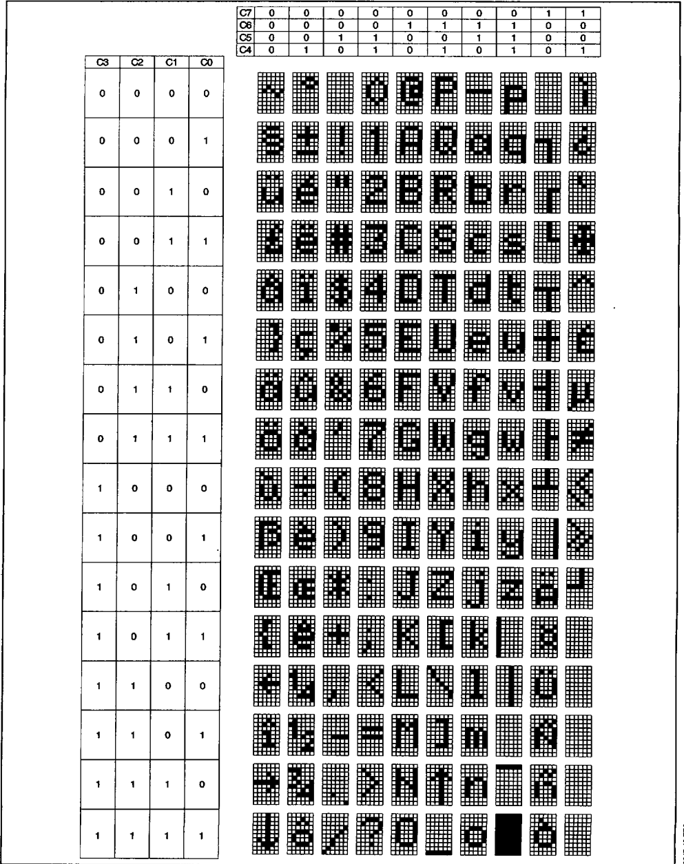
Figure 35 : GOE Alphanumeric Character Set in 80 Character/Row Mode - TS9347
