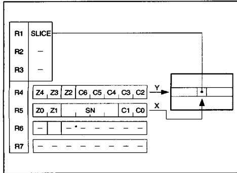
Figure 25 : Accessing a Character Slice in Memory
