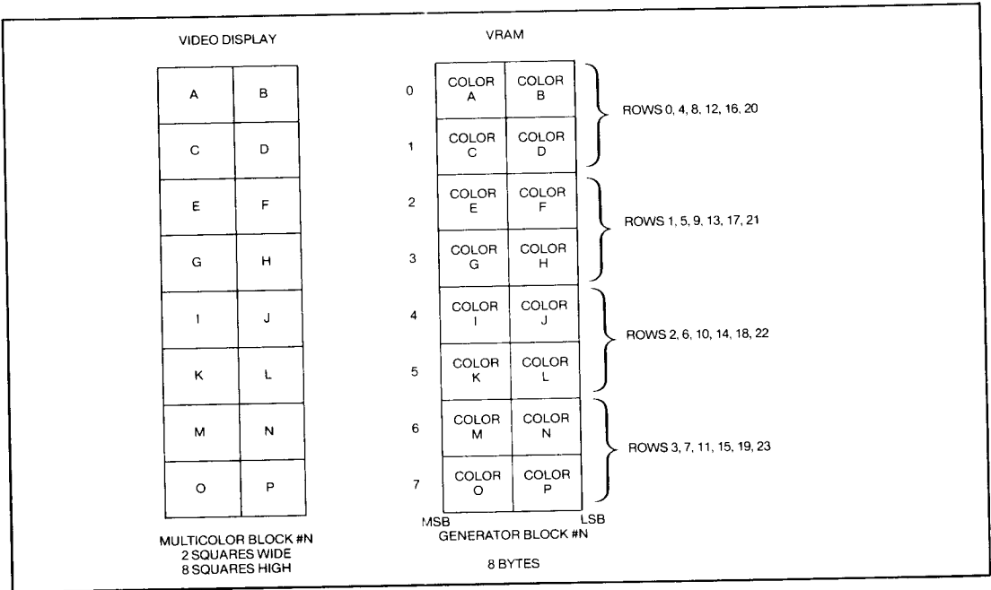
Figure 15. MULTICOLOR BLOCK DISPLAY
