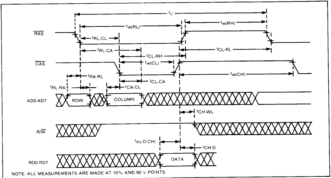
Figure 34. VRAM READ CYCLE
