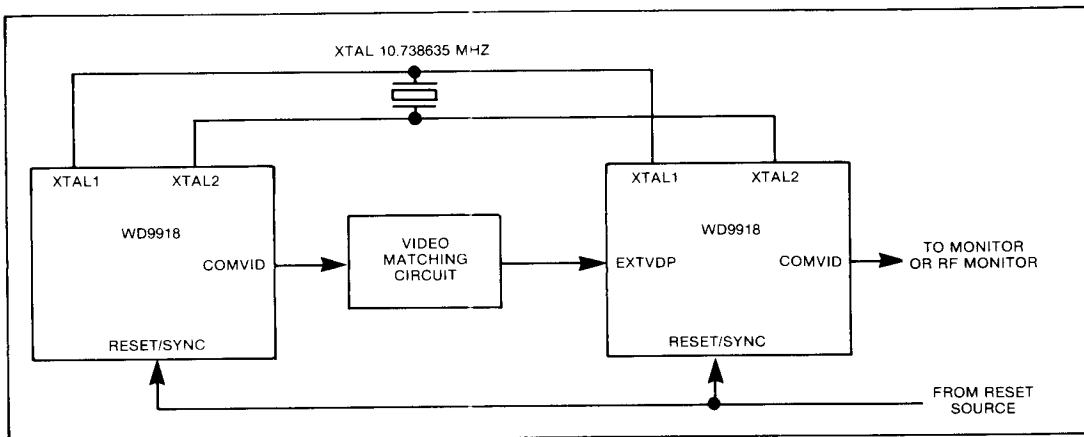
Figure 27. CASCADING TWO WD9918 VDPs
