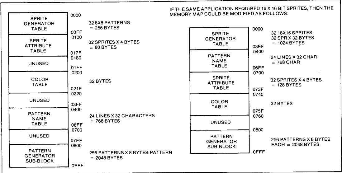
Figure 24. VDP-VRAM MEMORY ALLOCATION
