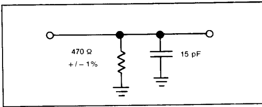
Figure 29. LOAD CIRCUIT FOR COMVID (ALL DEVICES) AND R-Y, Y, B-Y SWITCHING CHARACTERISTICS (WD9928/9929)
