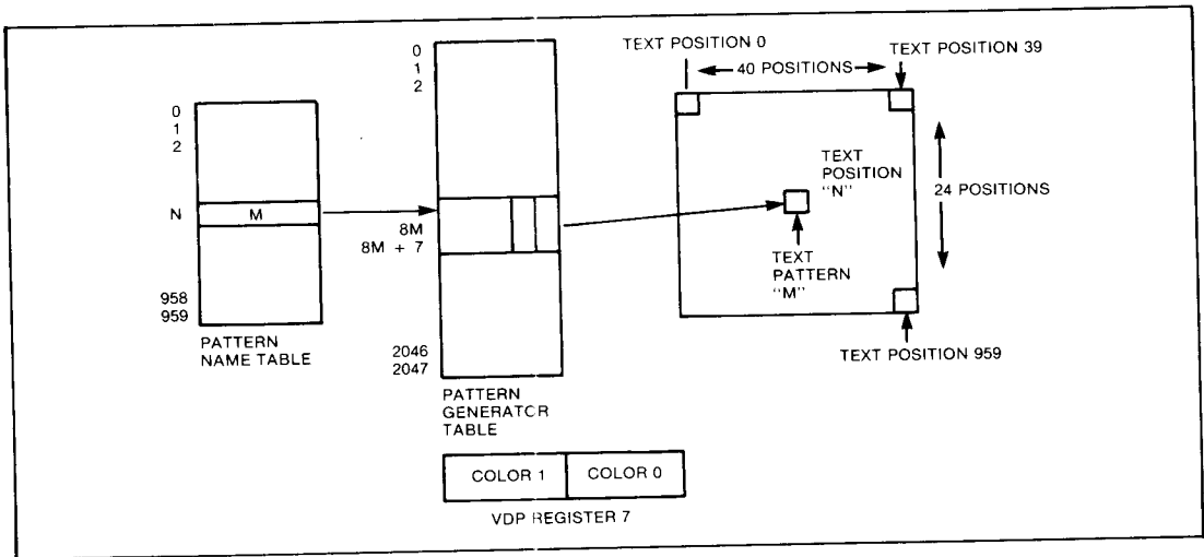
Figure 18. MAPPING OF VRAM INTO THE PATTERN PLANE IN TEXT MODE
