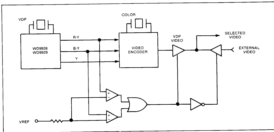
Figure 8. USING COLOR DIFFERENCE SIGNALS TO MIX EXTERNAL VIDEO SOURCES
