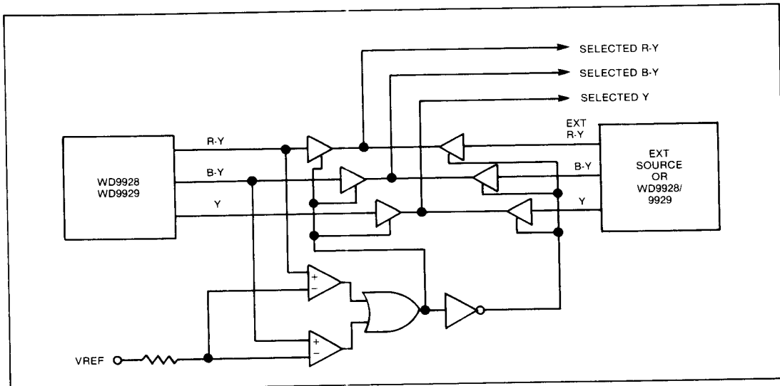
Figure 7. USING COLOR DIFFERENCE SIGNALS TO MIX EXTERNAL COLOR DIFFERENCE TYPE SOURCE
