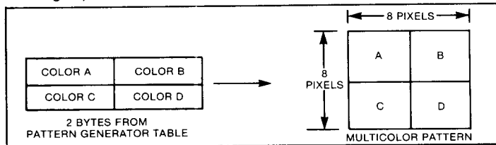
Figure 14. MULTICOLOR LIST MAPPING
