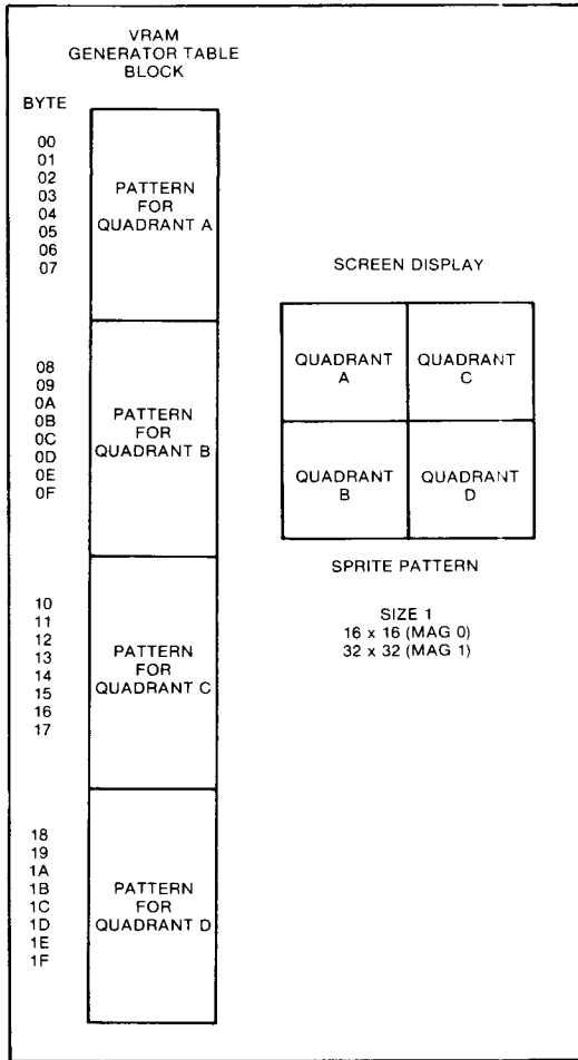
Figure 21. SIZE 1 SPRITE MAPPING
