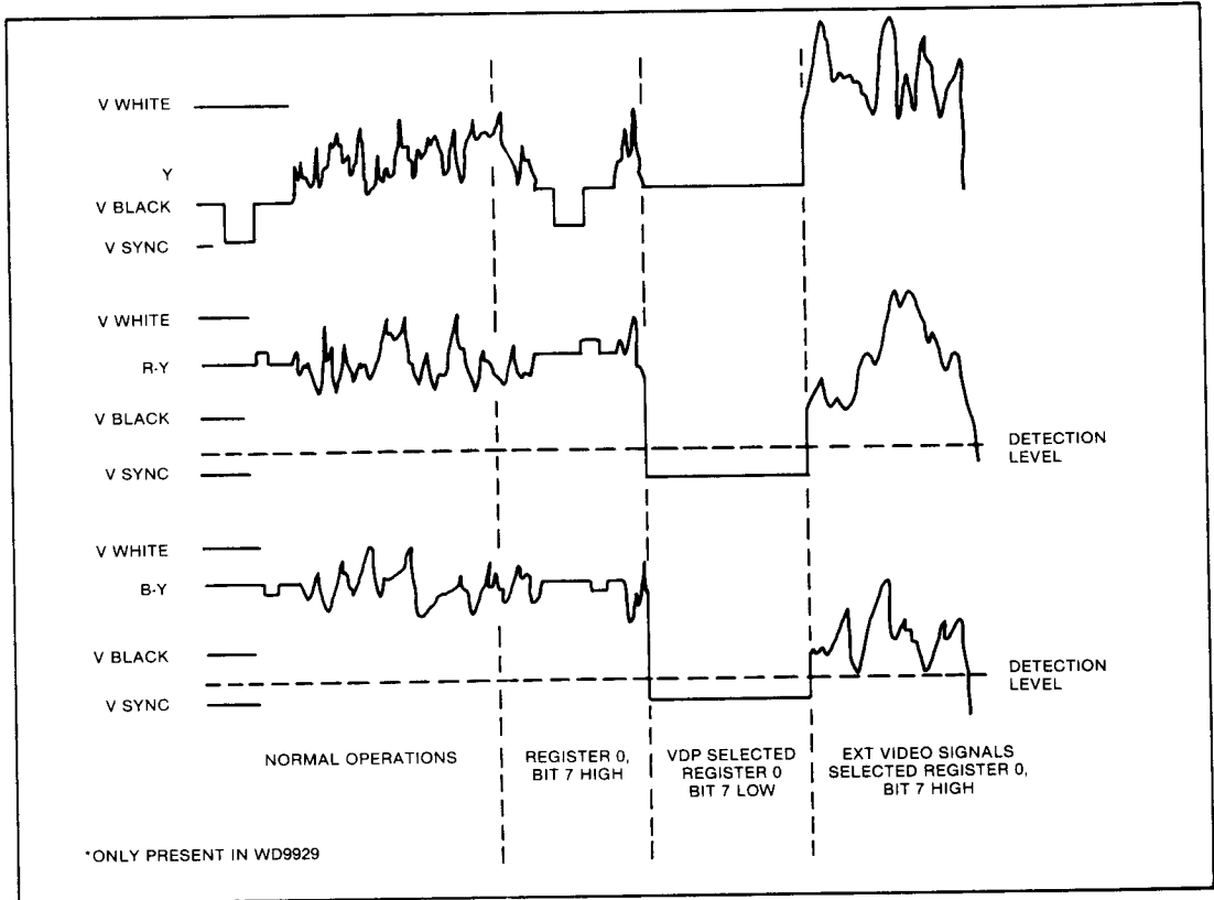
Figure 6. WD9928/9929 SIGNAL WAVEFORMS FOR MULTIPLE VDP OPERATION
