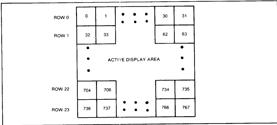
Figure 9. PATTERN GRAPHICS NAME TABLE MAPPING
