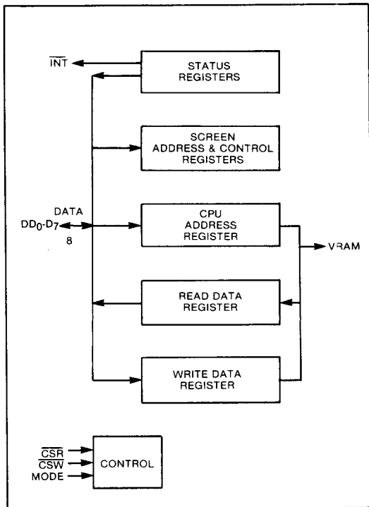
Figure 3. VDP TO CPU INTERFACE
