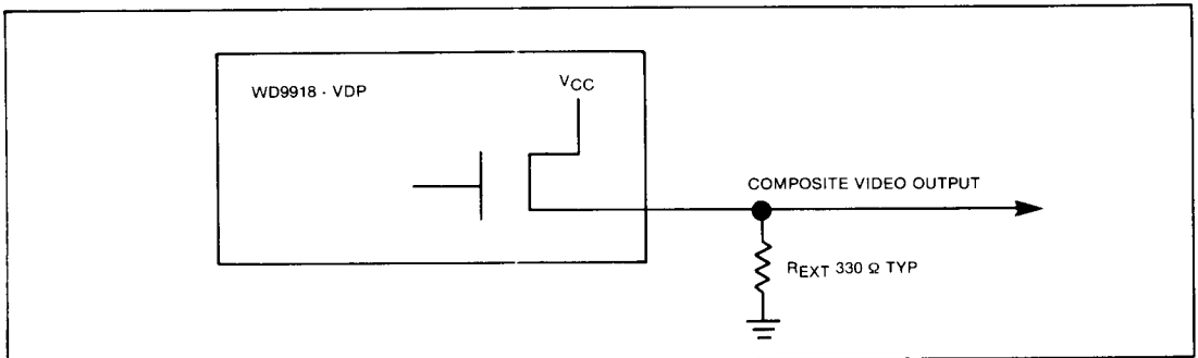
Figure 25. COMPOSITE VIDEO PULL-DOWN CIRCUIT
