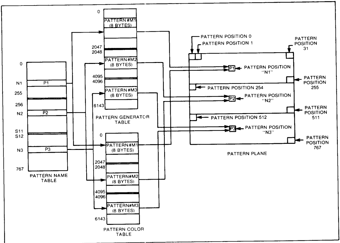
Figure 12. GRAPHICS II MODE MAPPING
