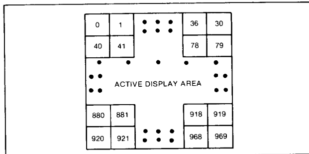
Figure 17. TEXT MODE NAME TABLE PATTERN POSITIONS
