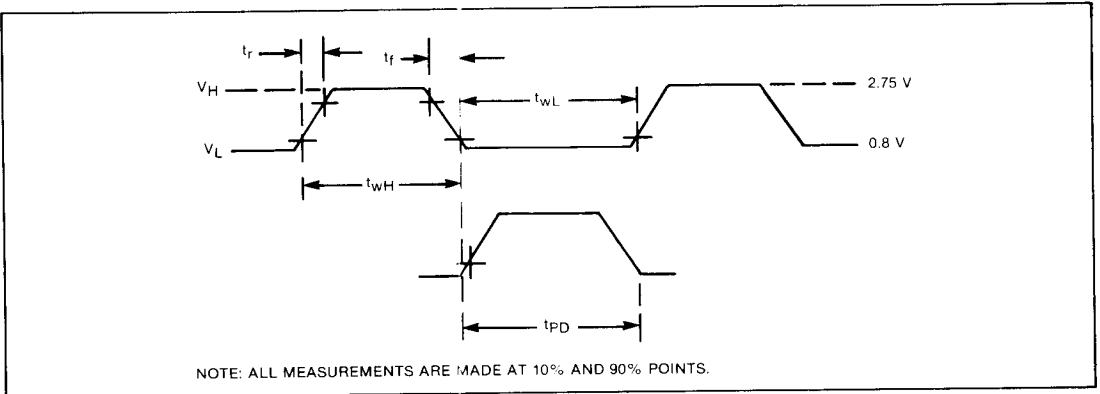
Figure 35. EXTERNAL CLOCK TIMING WAVEFORM
