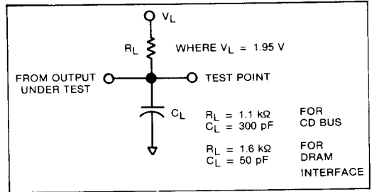
Figure 30. LOAD CIRCUITS FOR ALL OUTPUTS EXCEPT COMVID, R-Y, Y, B-Y
