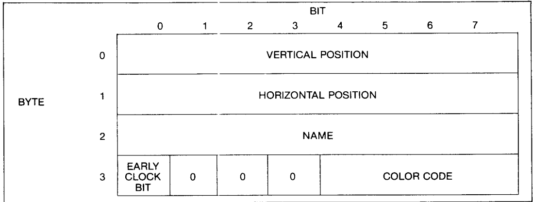
Figure 19. SPRITE ATTRIBUTE TABLE ENTRY
