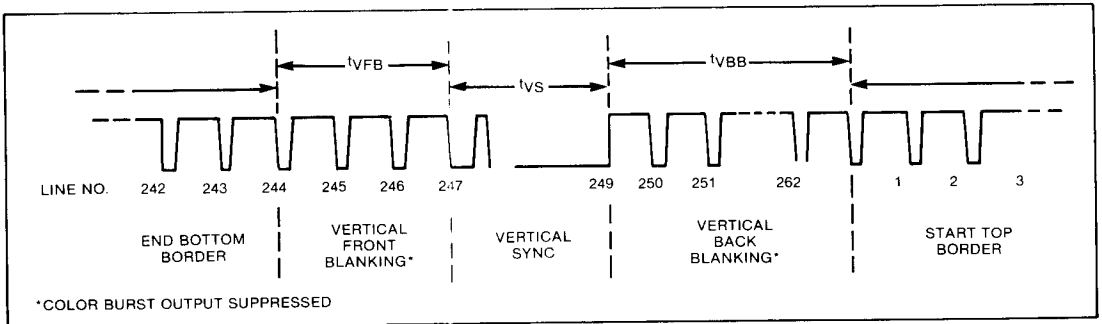
Figure 37. WD9918 VERTICAL TIMING
