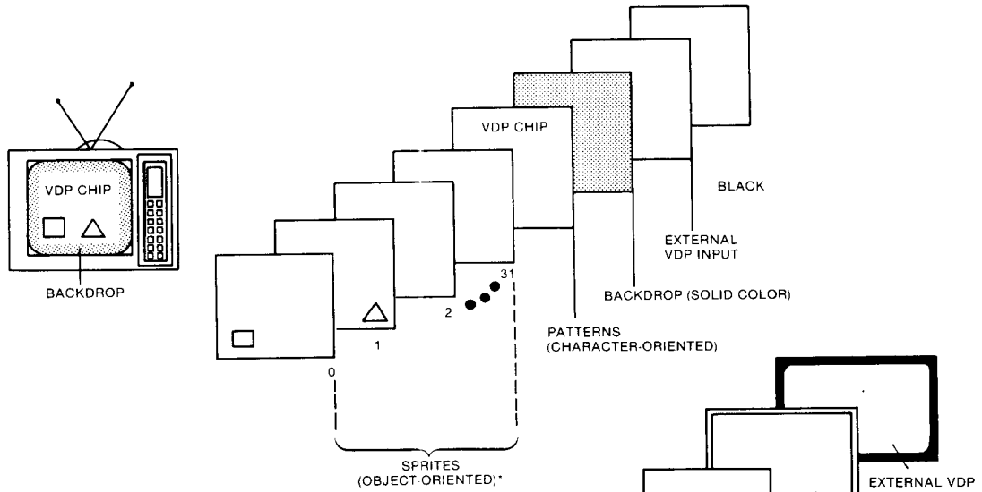
Figure 4. VDP DISPLAY PLANES (DEFINITION)
