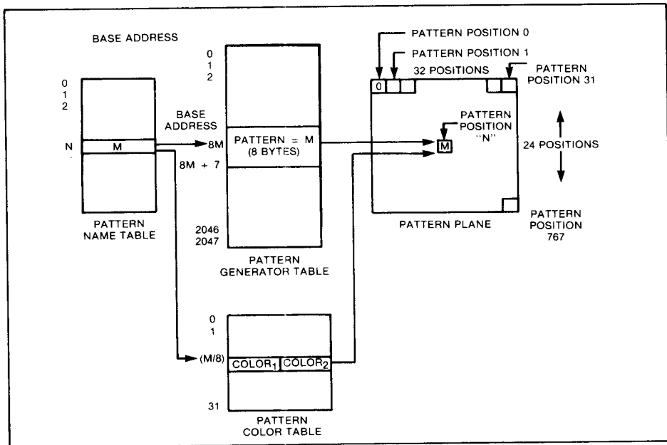
Figure 10. GRAPHICS I MODE MAPPING
