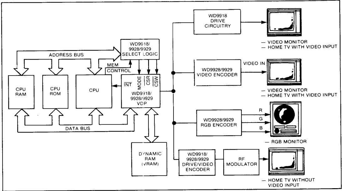
Figure 1. WD9918/28/29 SYSTEM BLOCK DIAGRAM
