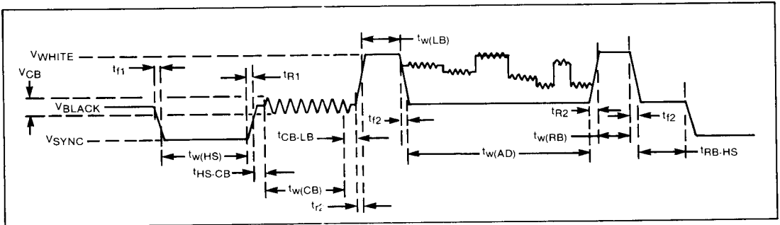
Figure 36. WD9918 COMVID HORIZONTAL TIMING
