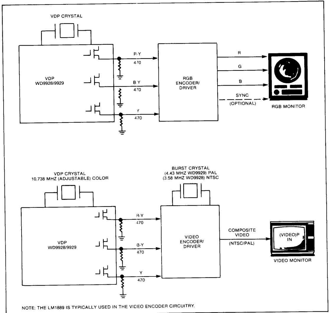
Figure 26. USE OF WD9928/9929 WITH DIFFERENT MONITORS
