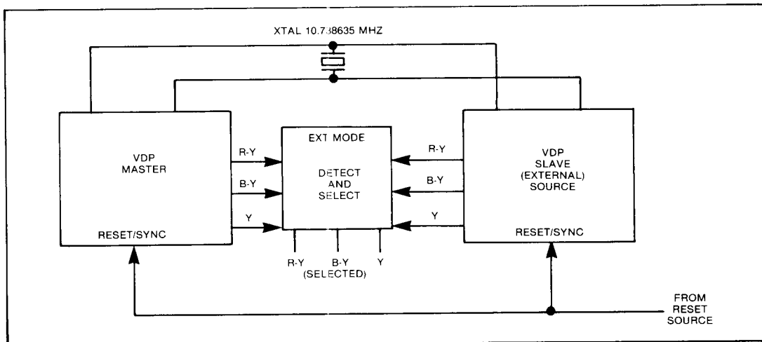
Figure 28. CASCADING TWO WD9918/9929 VDPs
