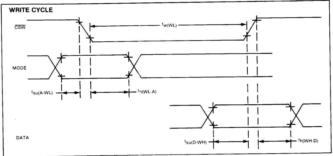
Figure 31. CPU - VDP WRITE CYCLE FOR WD9918/9928/9929
