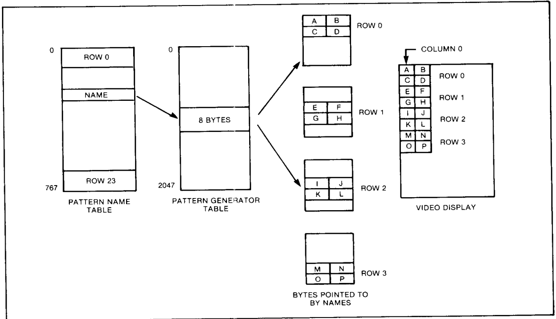
Figure 16. MULTICOLOR MODE MAPPING
