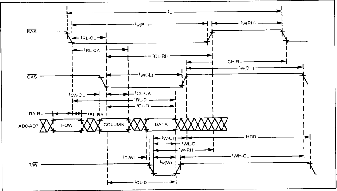
Figure 33. VRAM WRITE CYCLE
