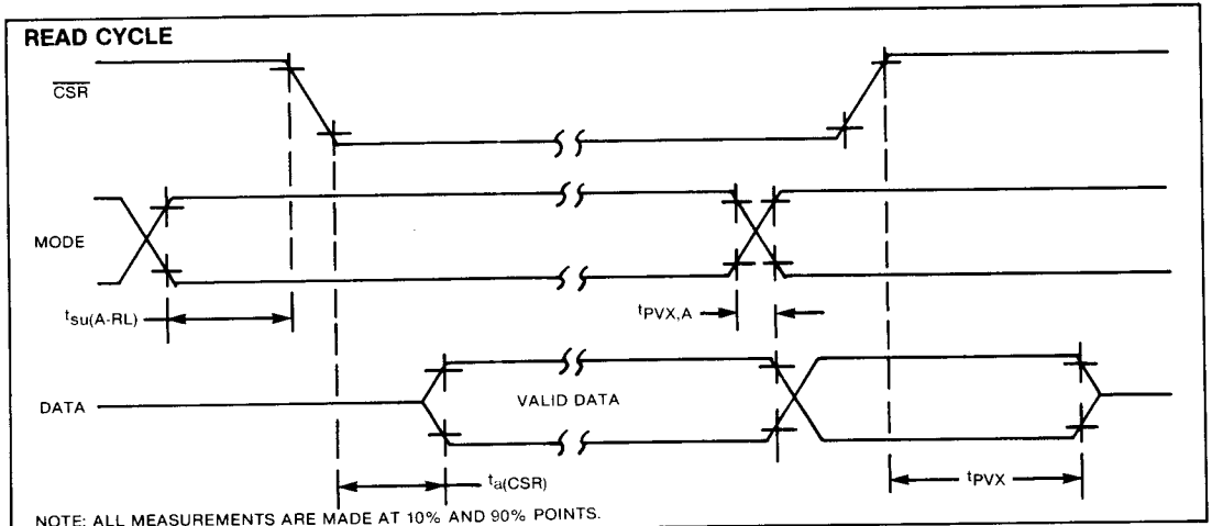
Figure 32. CPU - VDP READ CYCLE FOR WD9918/9928/9929
