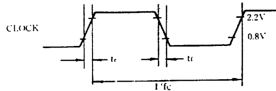
Fig. 1 Clock timing
