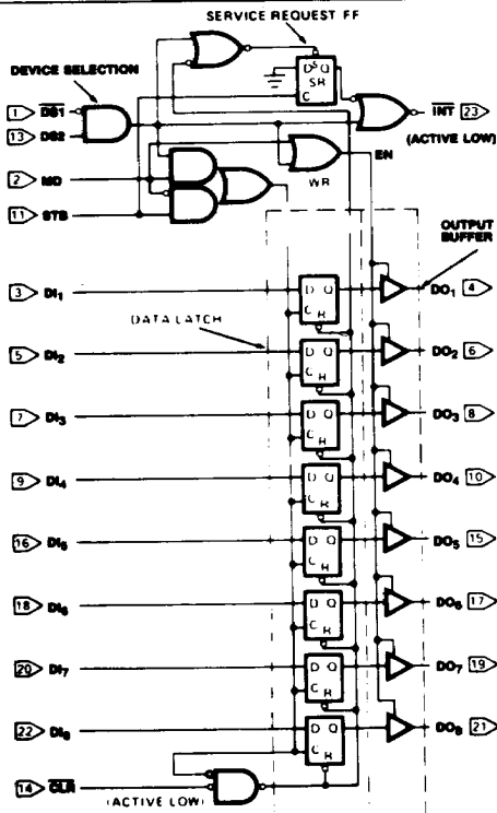
Figure 1. Logic Diagram
